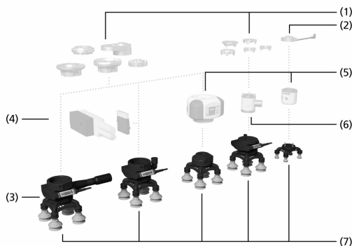
System design Lightweight Gripping Systems SLG
