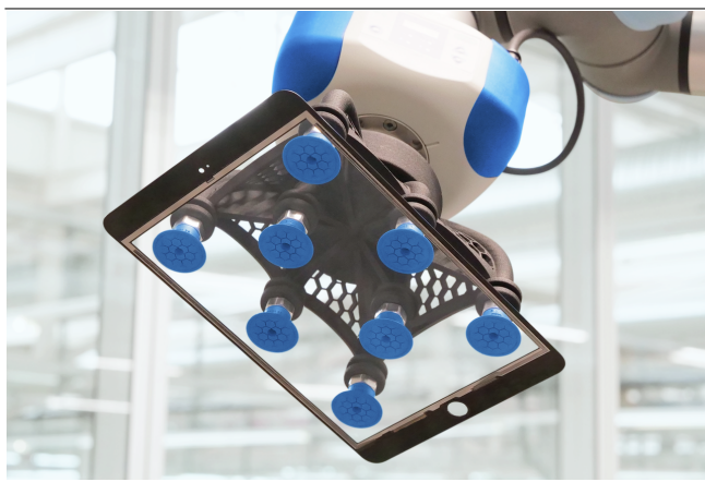
Lightweight gripper SLG with vacuum cups leaving few marks for handling display glass
